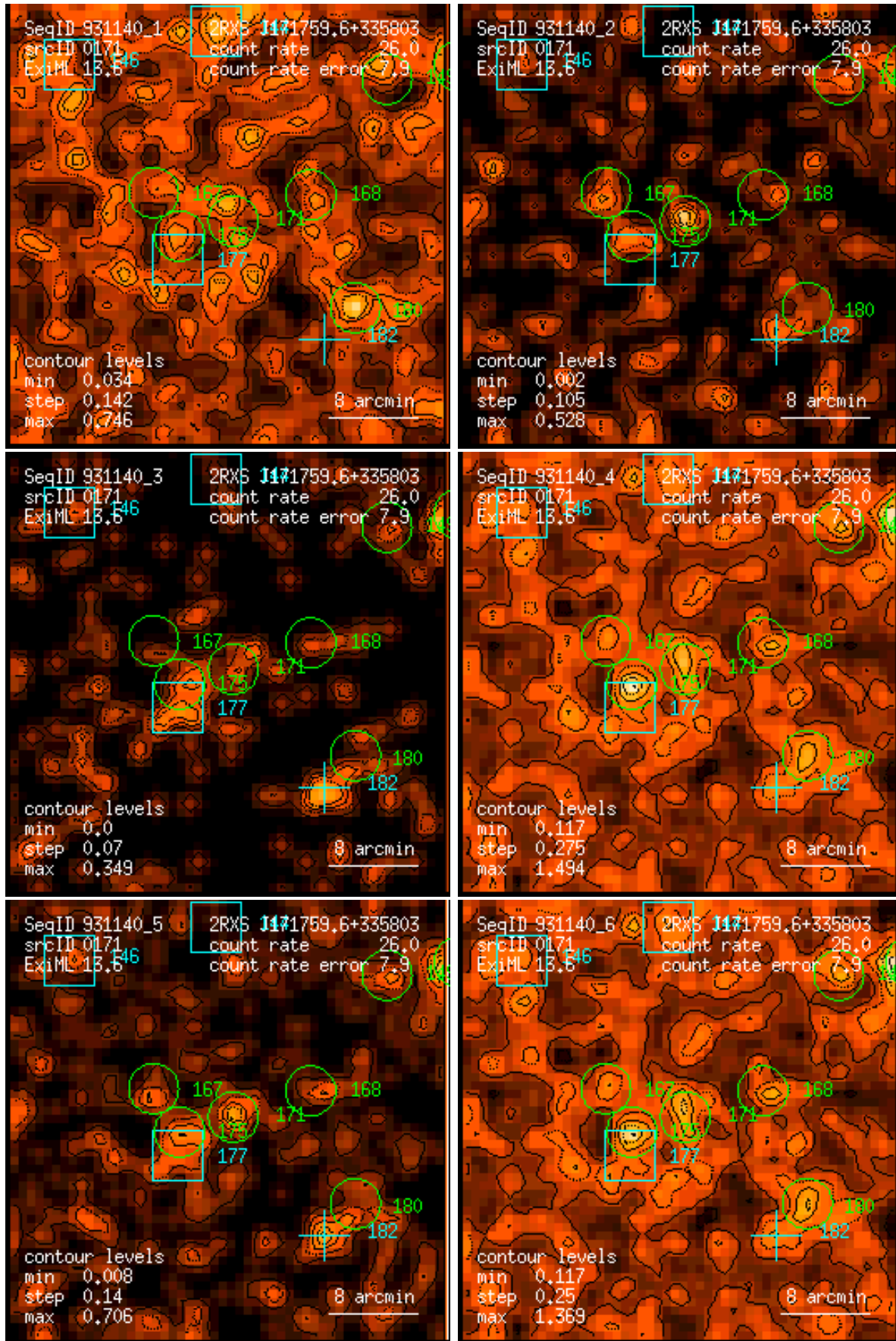
Figure 171: RASS 931140: detection 0171: band rate images, Gaussian filter: (1) PSPC channels 11 – 41, (2) 52 – 90, (3) 91 – 201, (4) 11 – 235, (5) 52 – 201, (6) 11 – 201. Broad band rates in counts/ks. Band rate contour levels in counts/ks/arcmin 2 .
