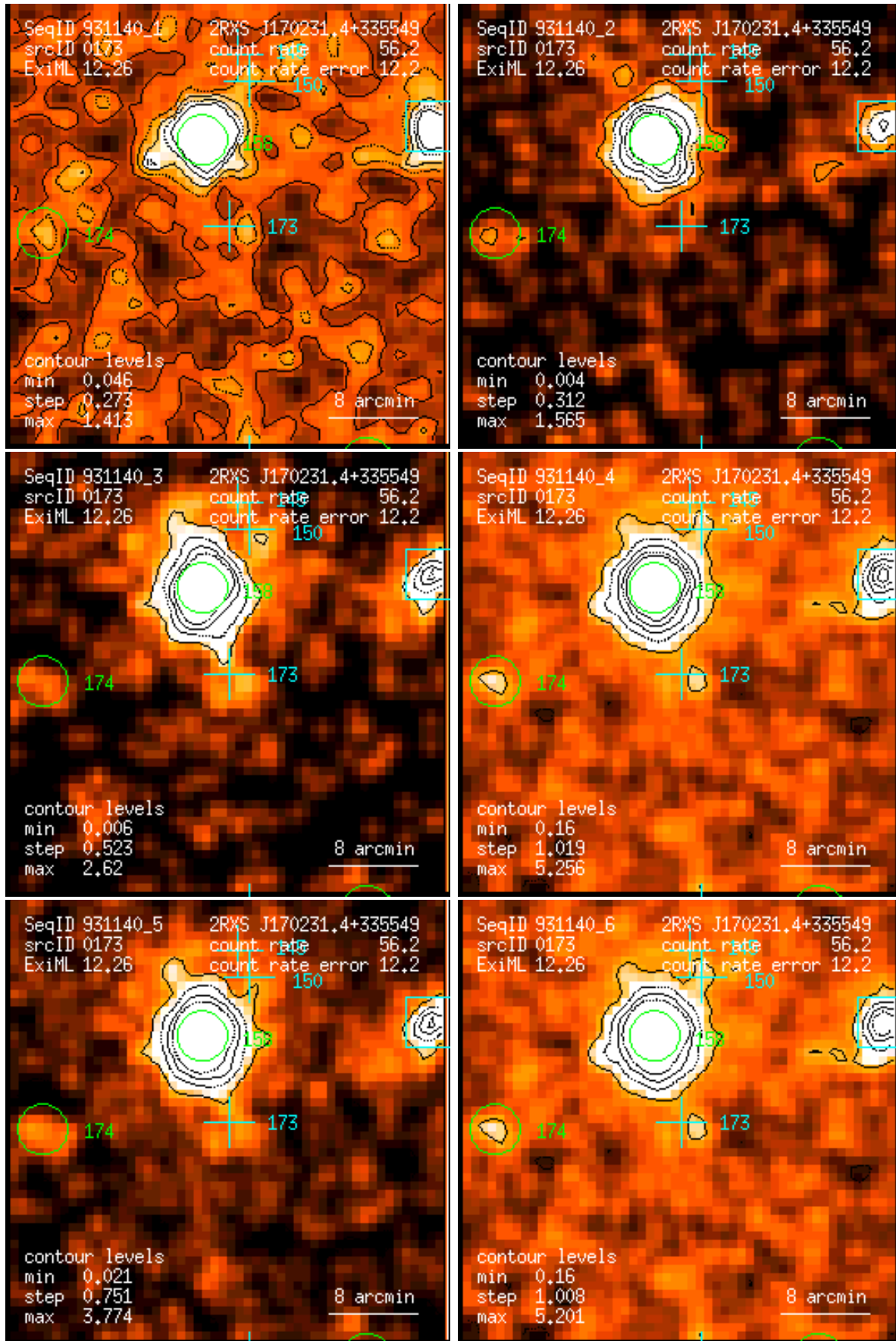
Figure 173: RASS 931140: detection 0173: band rate images, Gaussian filter: (1) PSPC channels 11 – 41, (2) 52 – 90, (3) 91 – 201, (4) 11 – 235, (5) 52 – 201, (6) 11 – 201. Broad band rates in counts/ks. Band rate contour levels in counts/ks/arcmin 2 .
