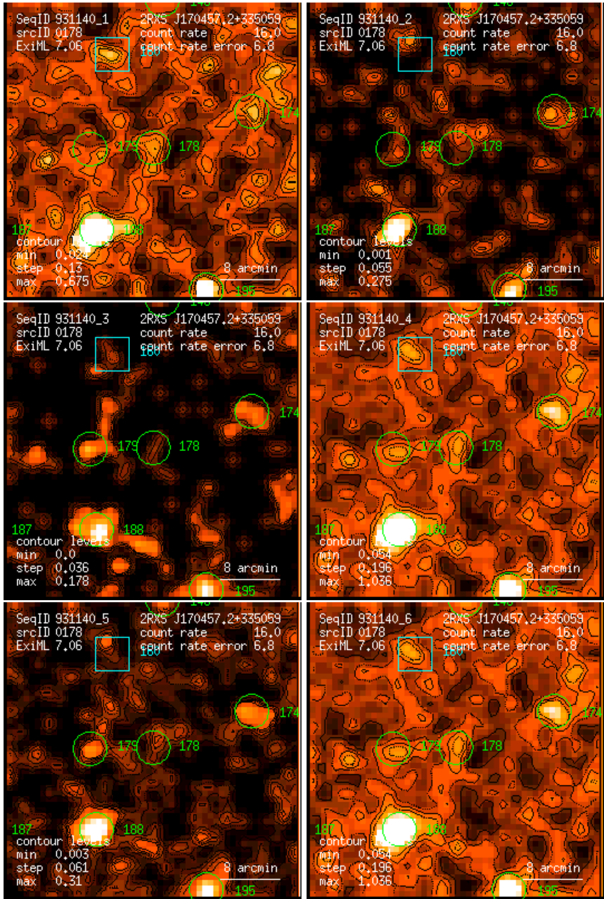
Figure 178: RASS 931140: detection 0178: band rate images, Gaussian filter: (1) PSPC channels 11 – 41, (2) 52 – 90, (3) 91 – 201, (4) 11 – 235, (5) 52 – 201, (6) 11 – 201. Broad band rates in counts/ks. Band rate contour levels in counts/ks/arcmin 2 .
