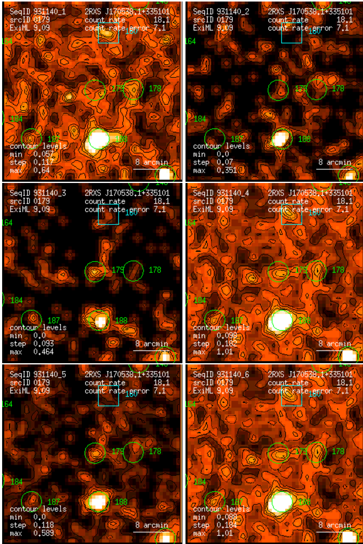
Figure 179: RASS 931140: detection 0179: band rate images, Gaussian filter: (1) PSPC channels 11 – 41, (2) 52 – 90, (3) 91 – 201, (4) 11 – 235, (5) 52 – 201, (6) 11 – 201. Broad band rates in counts/ks. Band rate contour levels in counts/ks/arcmin 2 .
