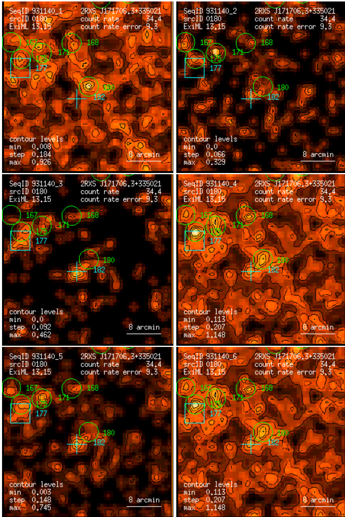
Figure 180: RASS 931140: detection 0180: band rate images, Gaussian filter: (1) PSPC channels 11 – 41, (2) 52 – 90, (3) 91 – 201, (4) 11 – 235, (5) 52 – 201, (6) 11 – 201. Broad band rates in counts/ks. Band rate contour levels in counts/ks/arcmin 2 .
