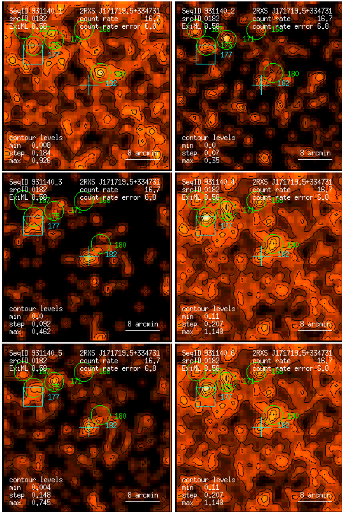
Figure 182: RASS 931140: detection 0182: band rate images, Gaussian filter: (1) PSPC channels 11 – 41, (2) 52 – 90, (3) 91 – 201, (4) 11 – 235, (5) 52 – 201, (6) 11 – 201. Broad band rates in counts/ks. Band rate contour levels in counts/ks/arcmin 2 .
