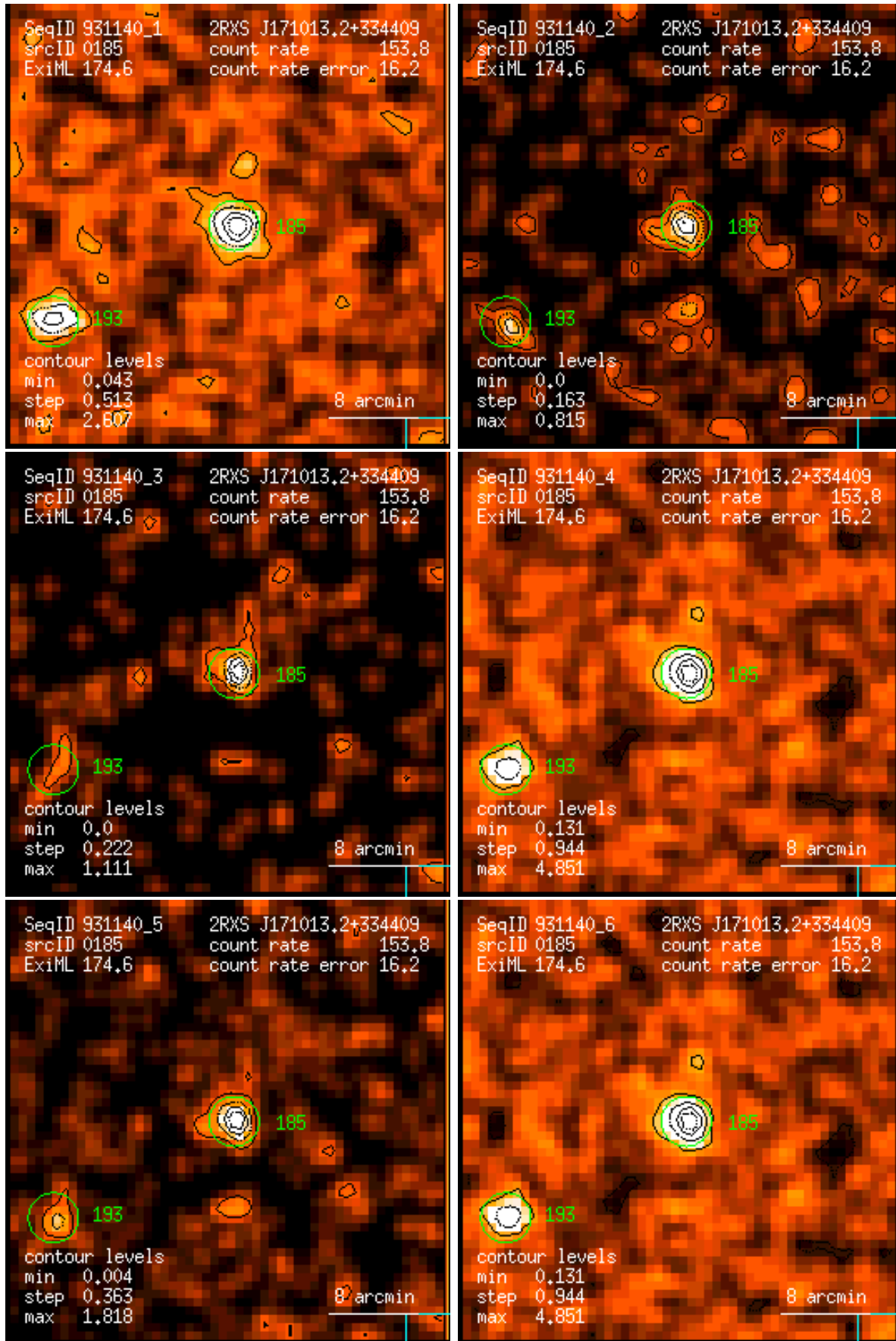
Figure 185: RASS 931140: detection 0185: band rate images, Gaussian filter: (1) PSPC channels 11 – 41, (2) 52 – 90, (3) 91 – 201, (4) 11 – 235, (5) 52 – 201, (6) 11 – 201. Broad band rates in counts/ks. Band rate contour levels in counts/ks/arcmin 2 .
