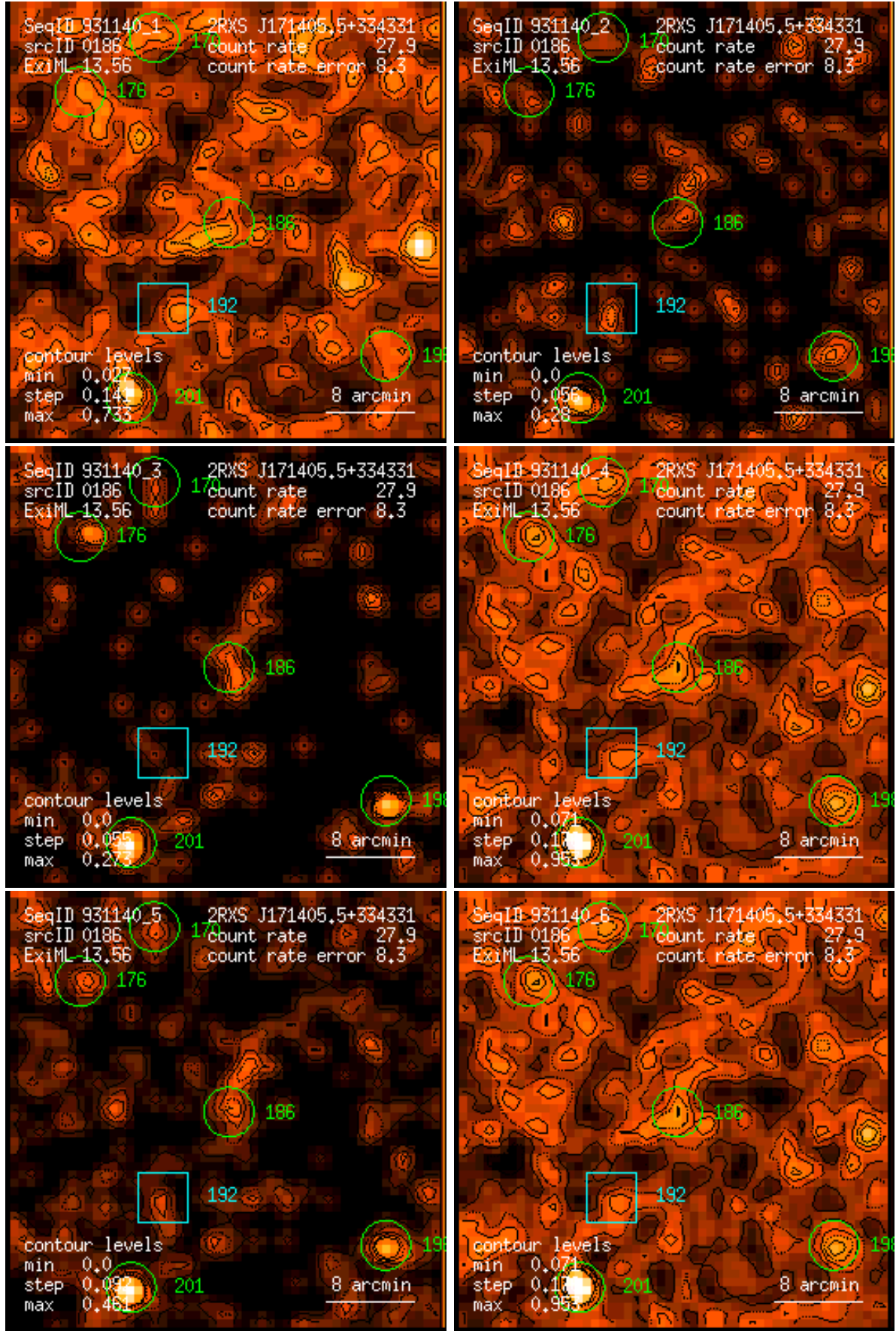
Figure 186: RASS 931140: detection 0186: band rate images, Gaussian filter: (1) PSPC channels 11 – 41, (2) 52 – 90, (3) 91 – 201, (4) 11 – 235, (5) 52 – 201, (6) 11 – 201. Broad band rates in counts/ks. Band rate contour levels in counts/ks/arcmin 2 .
