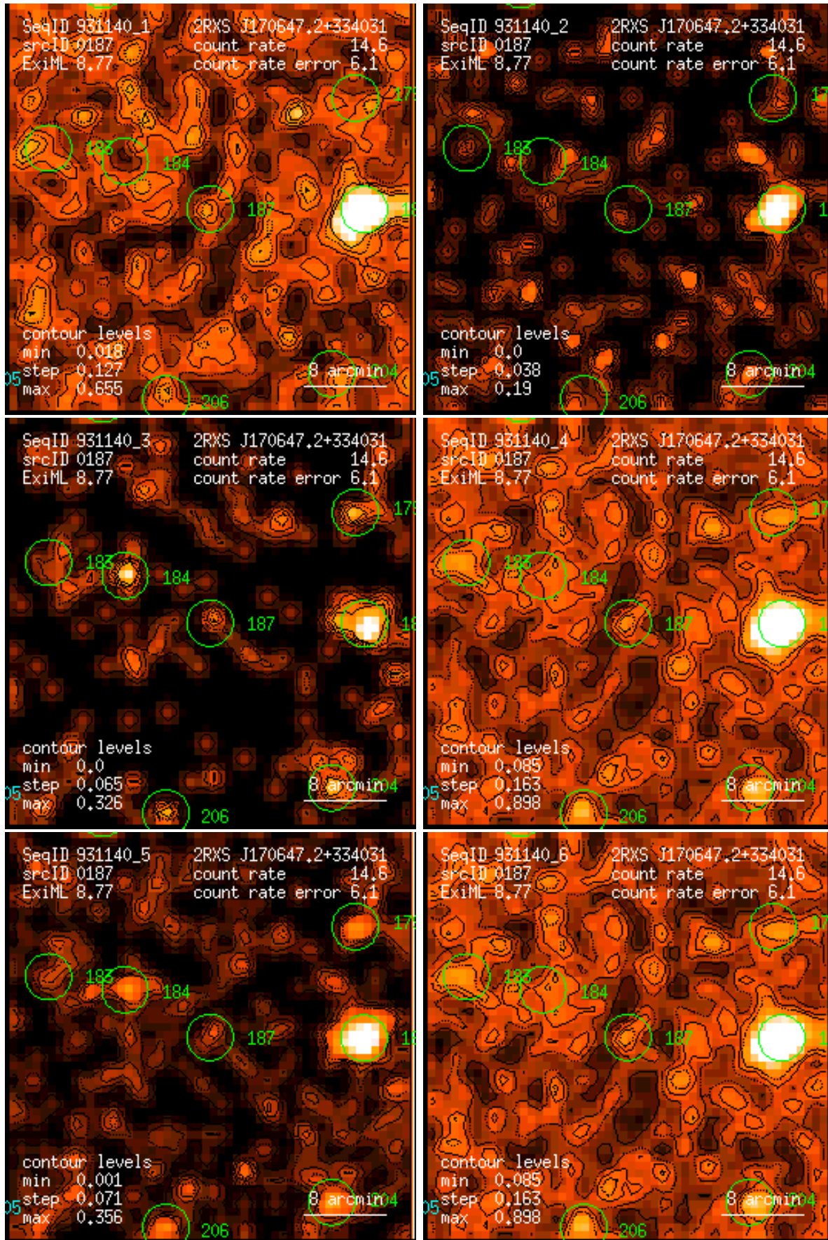
Figure 187: RASS 931140: detection 0187: band rate images, Gaussian filter: (1) PSPC channels 11 – 41, (2) 52 – 90, (3) 91 – 201, (4) 11 – 235, (5) 52 – 201, (6) 11 – 201. Broad band rates in counts/ks. Band rate contour levels in counts/ks/arcmin 2 .
