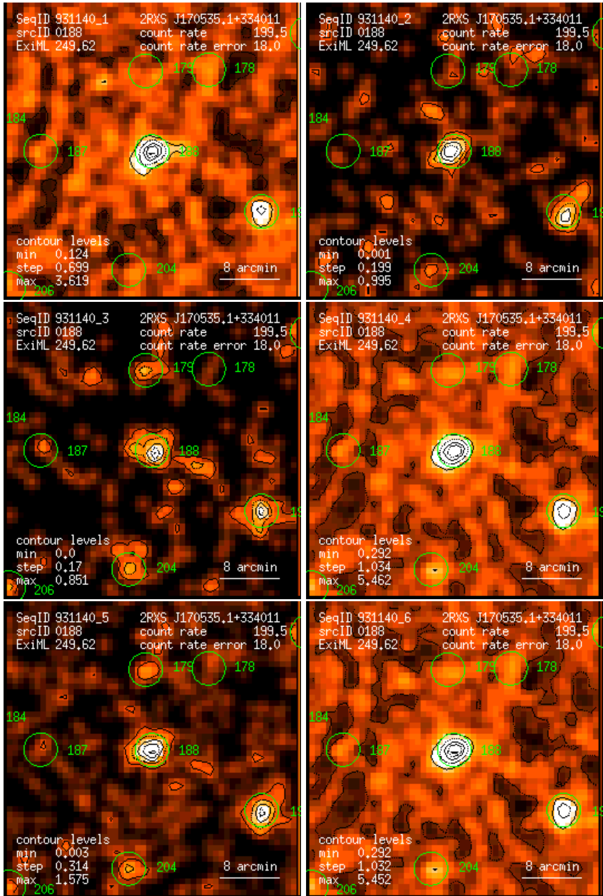
Figure 188: RASS 931140: detection 0188: band rate images, Gaussian filter: (1) PSPC channels 11 – 41, (2) 52 – 90, (3) 91 – 201, (4) 11 – 235, (5) 52 – 201, (6) 11 – 201. Broad band rates in counts/ks. Band rate contour levels in counts/ks/arcmin 2 .
