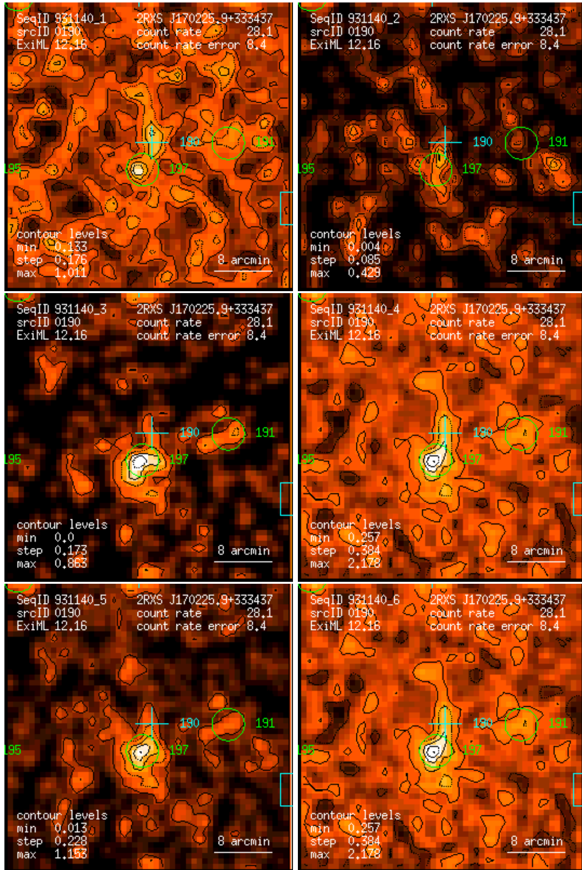
Figure 190: RASS 931140: detection 0190: band rate images, Gaussian filter: (1) PSPC channels 11 – 41, (2) 52 – 90, (3) 91 – 201, (4) 11 – 235, (5) 52 – 201, (6) 11 – 201. Broad band rates in counts/ks. Band rate contour levels in counts/ks/arcmin 2 .
