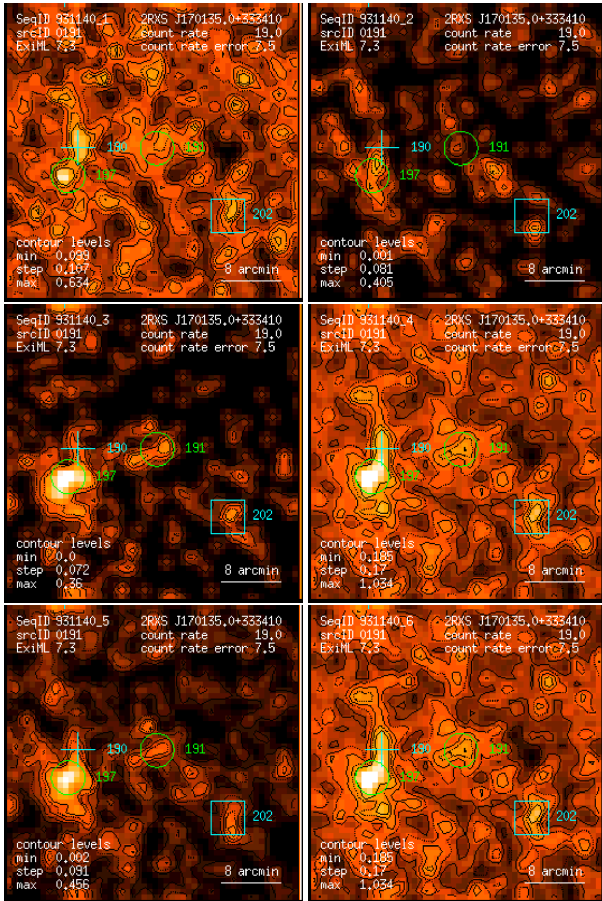
Figure 191: RASS 931140: detection 0191: band rate images, Gaussian filter: (1) PSPC channels 11 – 41, (2) 52 – 90, (3) 91 – 201, (4) 11 – 235, (5) 52 – 201, (6) 11 – 201. Broad band rates in counts/ks. Band rate contour levels in counts/ks/arcmin 2 .
