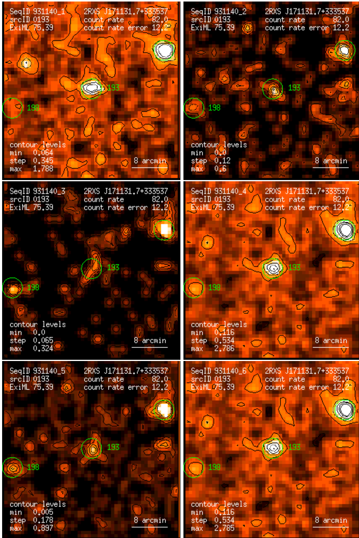
Figure 193: RASS 931140: detection 0193: band rate images, Gaussian filter: (1) PSPC channels 11 – 41, (2) 52 – 90, (3) 91 – 201, (4) 11 – 235, (5) 52 – 201, (6) 11 – 201. Broad band rates in counts/ks. Band rate contour levels in counts/ks/arcmin 2 .
