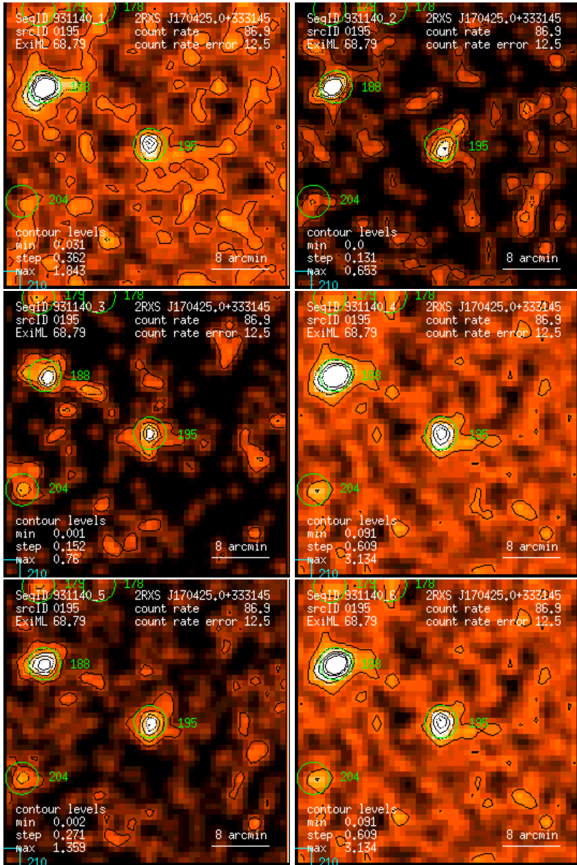
Figure 195: RASS 931140: detection 0195: band rate images, Gaussian filter: (1) PSPC channels 11 – 41, (2) 52 – 90, (3) 91 – 201, (4) 11 – 235, (5) 52 – 201, (6) 11 – 201. Broad band rates in counts/ks. Band rate contour levels in counts/ks/arcmin 2 .
