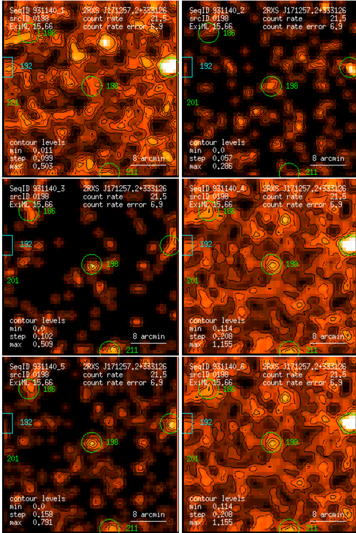
Figure 198: RASS 931140: detection 0198: band rate images, Gaussian filter: (1) PSPC channels 11 – 41, (2) 52 – 90, (3) 91 – 201, (4) 11 – 235, (5) 52 – 201, (6) 11 – 201. Broad band rates in counts/ks. Band rate contour levels in counts/ks/arcmin 2 .
