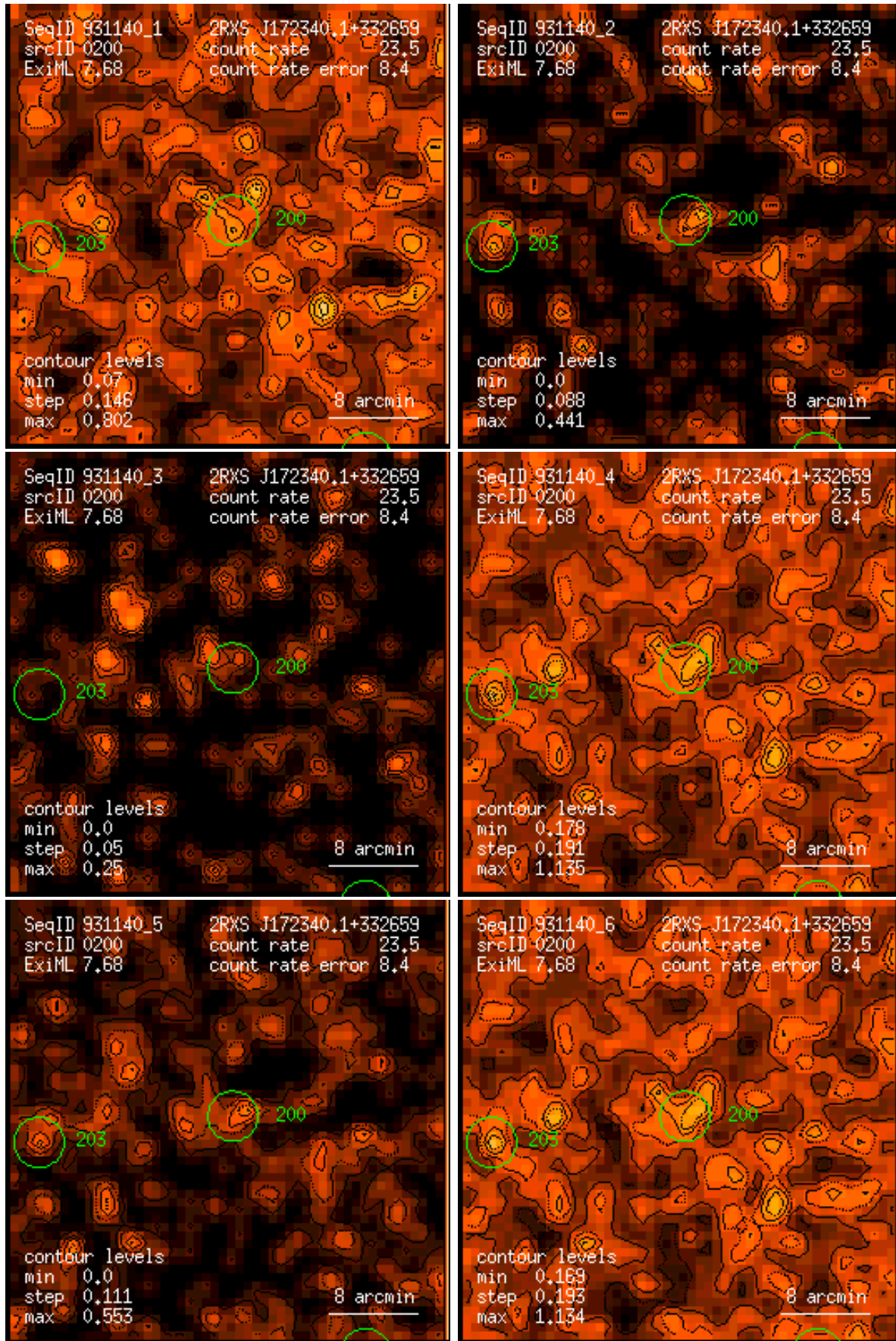
Figure 200: RASS 931140: detection 0200: band rate images, Gaussian filter: (1) PSPC channels 11 – 41, (2) 52 – 90, (3) 91 – 201, (4) 11 – 235, (5) 52 – 201, (6) 11 – 201. Broad band rates in counts/ks. Band rate contour levels in counts/ks/arcmin 2 .
