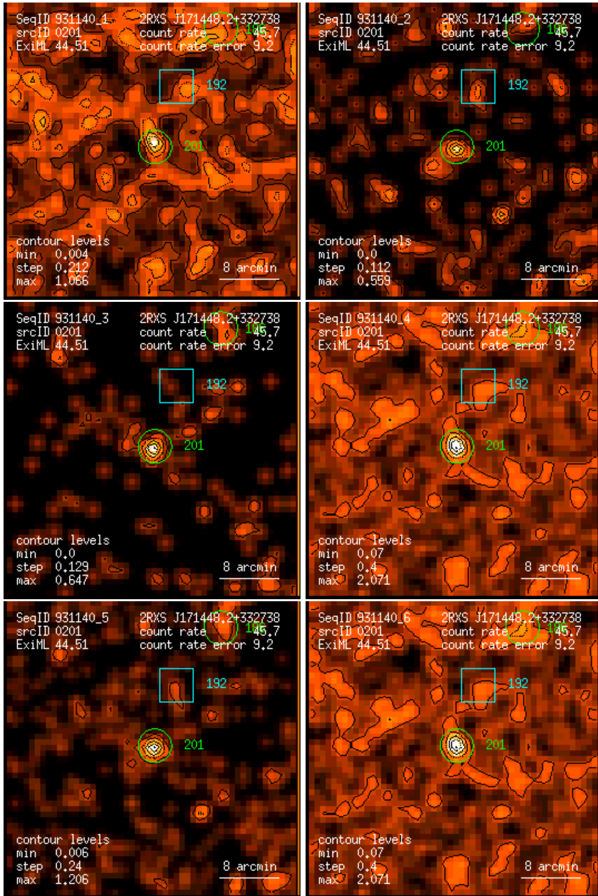
Figure 201: RASS 931140: detection 0201: band rate images, Gaussian filter: (1) PSPC channels 11 – 41, (2) 52 – 90, (3) 91 – 201, (4) 11 – 235, (5) 52 – 201, (6) 11 – 201. Broad band rates in counts/ks. Band rate contour levels in counts/ks/arcmin 2 .
