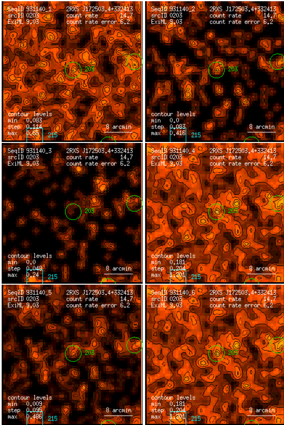
Figure 203: RASS 931140: detection 0203: band rate images, Gaussian filter: (1) PSPC channels 11 – 41, (2) 52 – 90, (3) 91 – 201, (4) 11 – 235, (5) 52 – 201, (6) 11 – 201. Broad band rates in counts/ks. Band rate contour levels in counts/ks/arcmin 2 .
