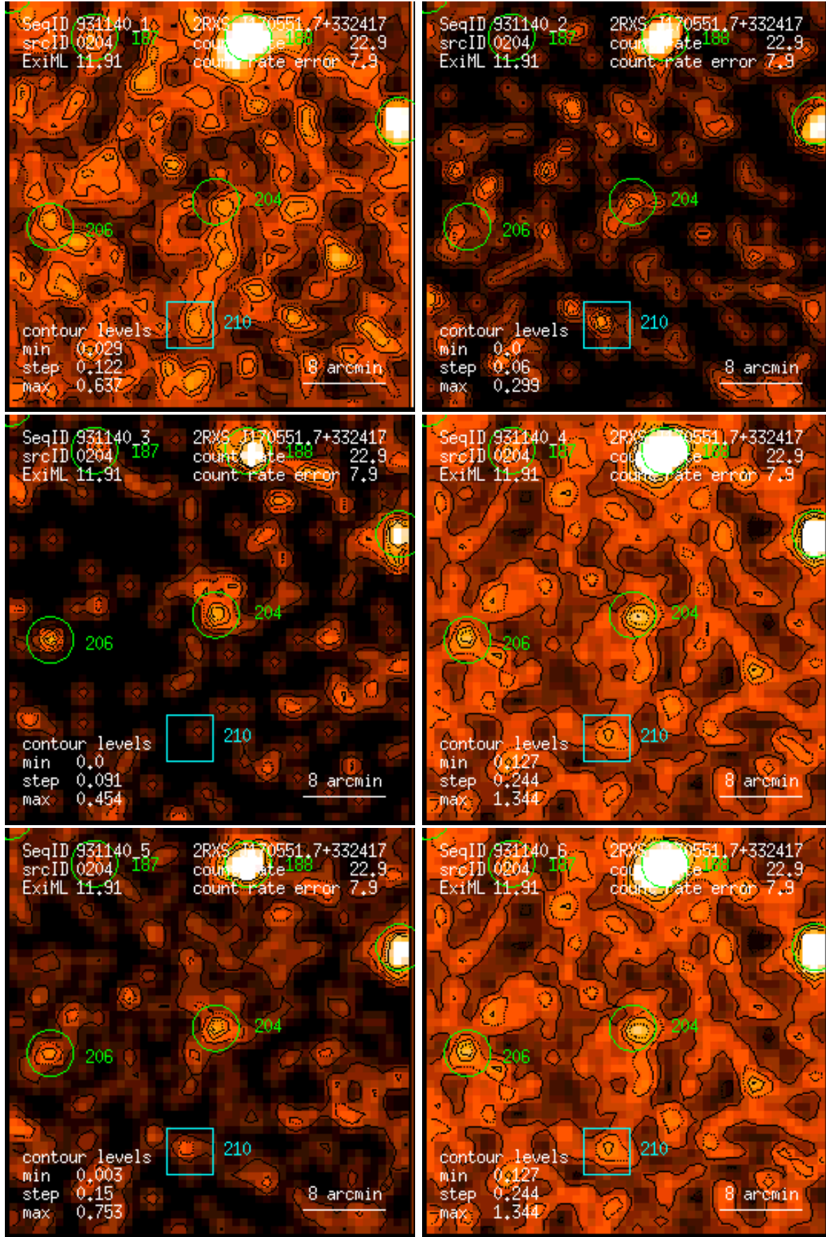
Figure 204: RASS 931140: detection 0204: band rate images, Gaussian filter: (1) PSPC channels 11 – 41, (2) 52 – 90, (3) 91 – 201, (4) 11 – 235, (5) 52 – 201, (6) 11 – 201. Broad band rates in counts/ks. Band rate contour levels in counts/ks/arcmin 2 .
