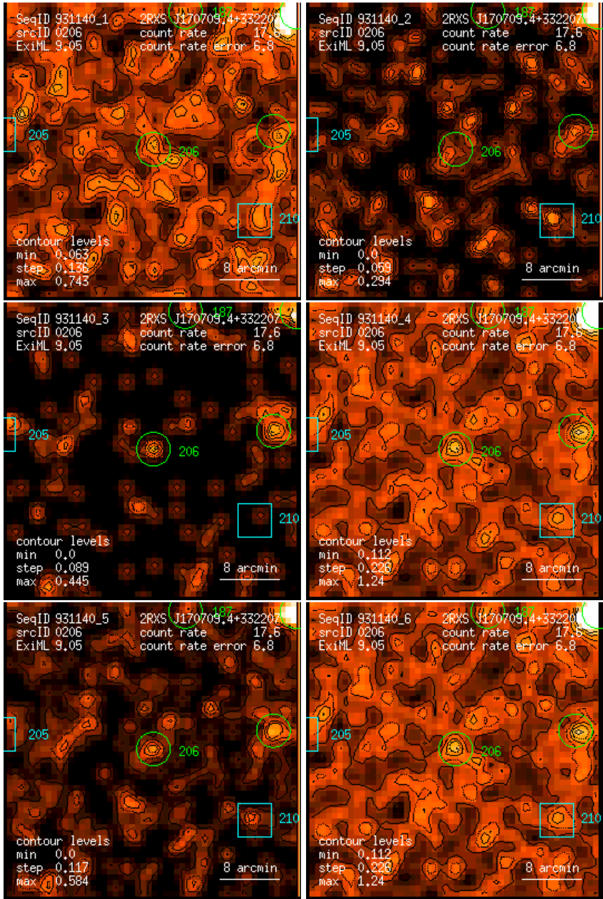
Figure 206: RASS 931140: detection 0206: band rate images, Gaussian filter: (1) PSPC channels 11 – 41, (2) 52 – 90, (3) 91 – 201, (4) 11 – 235, (5) 52 – 201, (6) 11 – 201. Broad band rates in counts/ks. Band rate contour levels in counts/ks/arcmin 2 .
