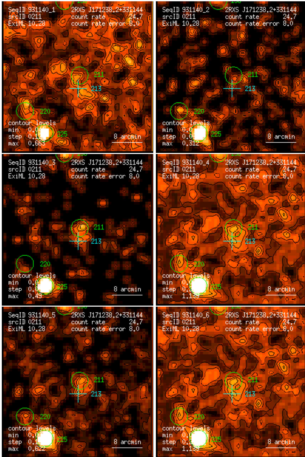
Figure 211: RASS 931140: detection 0211: band rate images, Gaussian filter: (1) PSPC channels 11 – 41, (2) 52 – 90, (3) 91 – 201, (4) 11 – 235, (5) 52 – 201, (6) 11 – 201. Broad band rates in counts/ks. Band rate contour levels in counts/ks/arcmin 2 .
