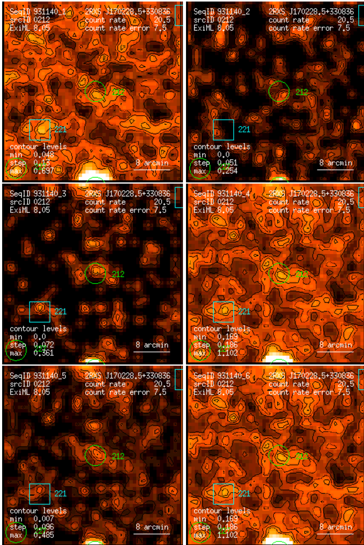
Figure 212: RASS 931140: detection 0212: band rate images, Gaussian filter: (1) PSPC channels 11 – 41, (2) 52 – 90, (3) 91 – 201, (4) 11 – 235, (5) 52 – 201, (6) 11 – 201. Broad band rates in counts/ks. Band rate contour levels in counts/ks/arcmin 2 .
