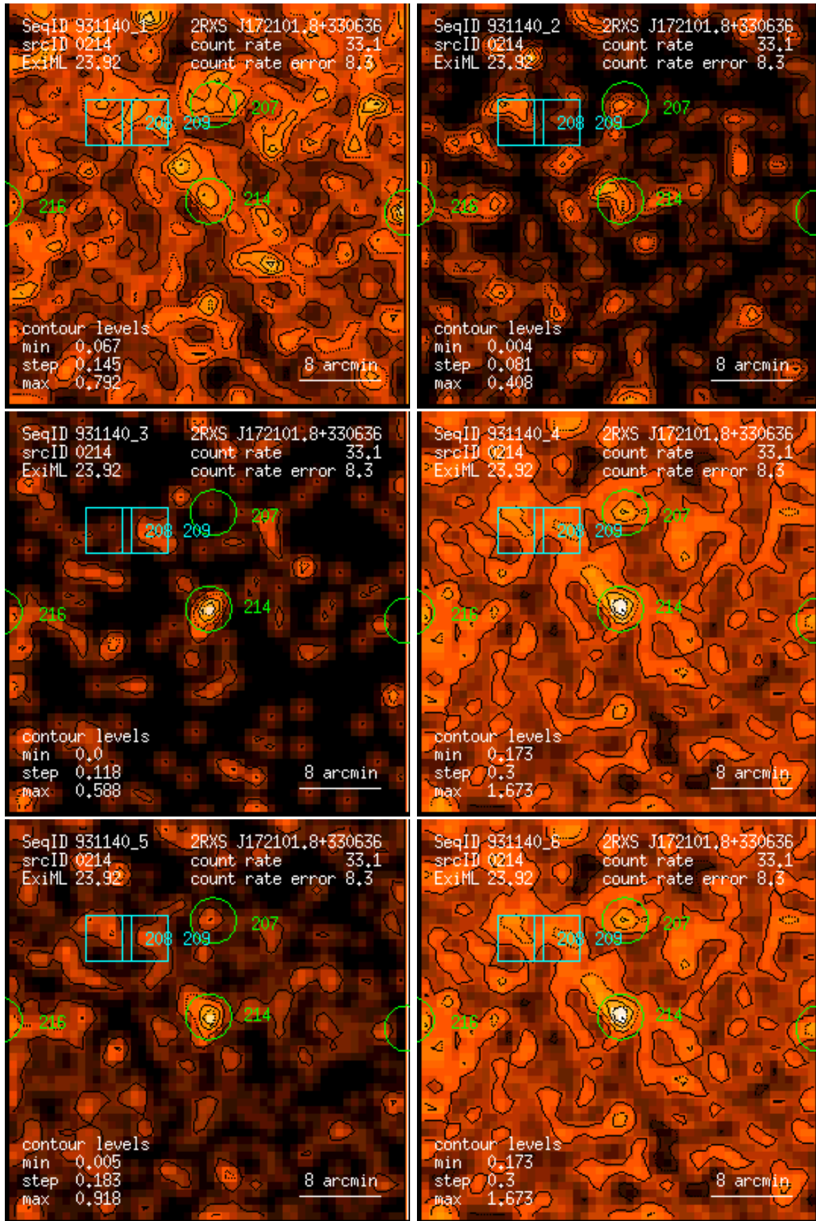
Figure 214: RASS 931140: detection 0214: band rate images, Gaussian filter: (1) PSPC channels 11 – 41, (2) 52 – 90, (3) 91 – 201, (4) 11 – 235, (5) 52 – 201, (6) 11 – 201. Broad band rates in counts/ks. Band rate contour levels in counts/ks/arcmin 2 .
