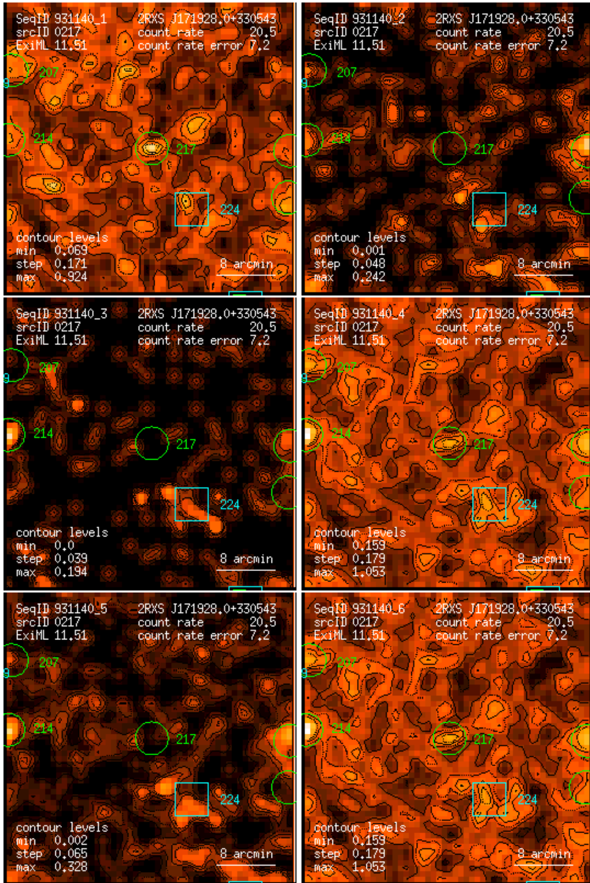
Figure 217: RASS 931140: detection 0217: band rate images, Gaussian filter: (1) PSPC channels 11 – 41, (2) 52 – 90, (3) 91 – 201, (4) 11 – 235, (5) 52 – 201, (6) 11 – 201. Broad band rates in counts/ks. Band rate contour levels in counts/ks/arcmin 2 .
