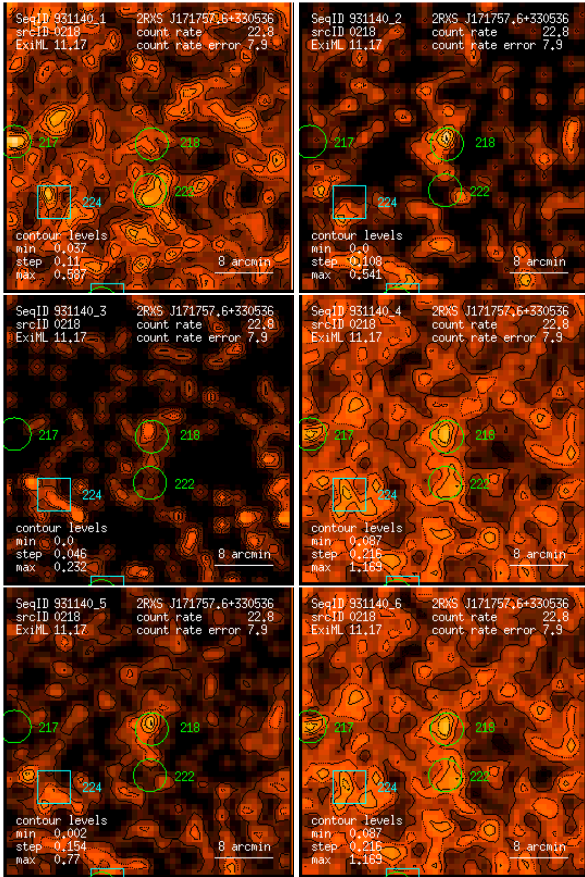
Figure 218: RASS 931140: detection 0218: band rate images, Gaussian filter: (1) PSPC channels 11 – 41, (2) 52 – 90, (3) 91 – 201, (4) 11 – 235, (5) 52 – 201, (6) 11 – 201. Broad band rates in counts/ks. Band rate contour levels in counts/ks/arcmin 2 .
