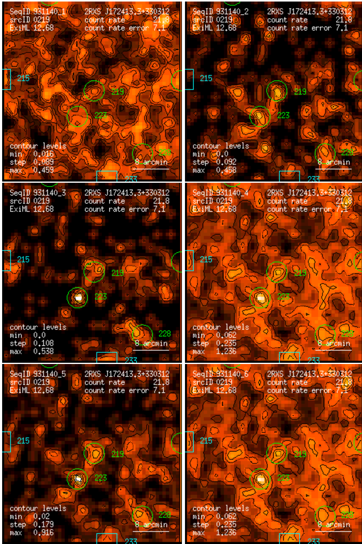
Figure 219: RASS 931140: detection 0219: band rate images, Gaussian filter: (1) PSPC channels 11 – 41, (2) 52 – 90, (3) 91 – 201, (4) 11 – 235, (5) 52 – 201, (6) 11 – 201. Broad band rates in counts/ks. Band rate contour levels in counts/ks/arcmin 2 .
