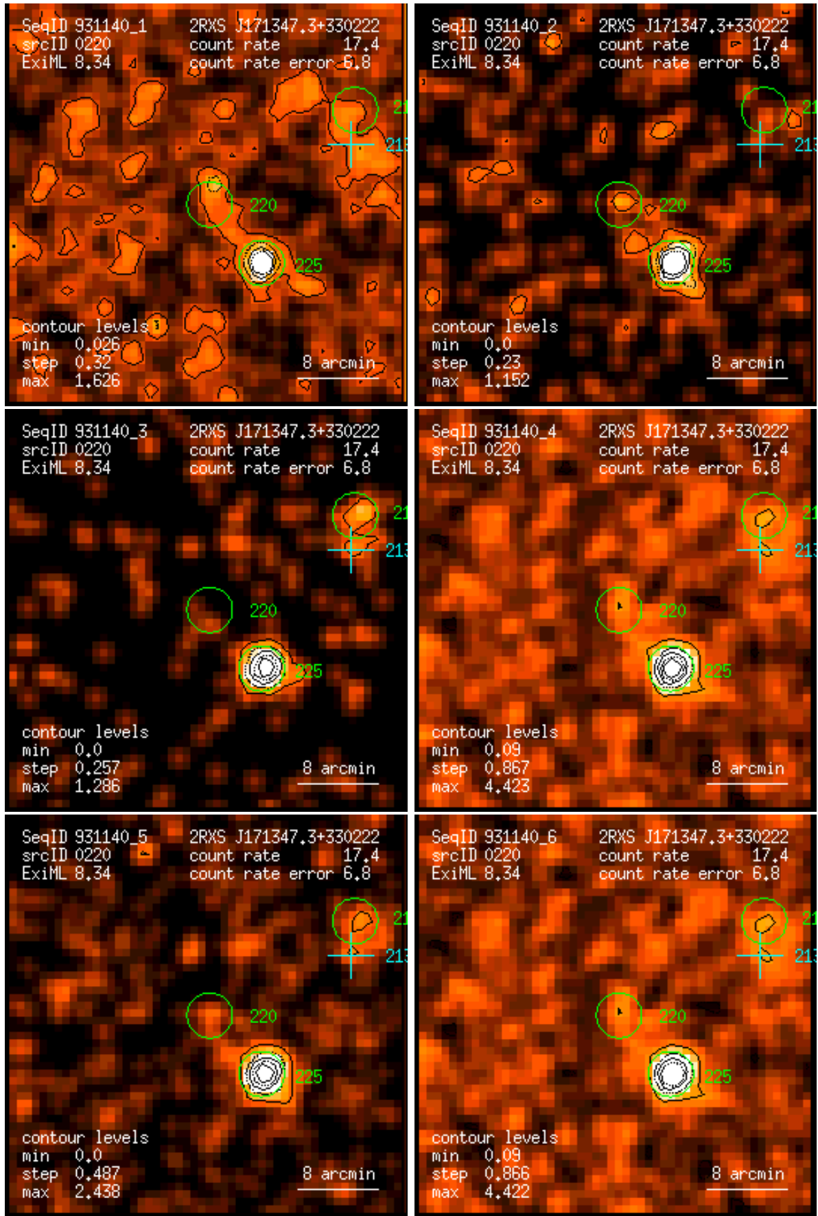
Figure 220: RASS 931140: detection 0220: band rate images, Gaussian filter: (1) PSPC channels 11 – 41, (2) 52 – 90, (3) 91 – 201, (4) 11 – 235, (5) 52 – 201, (6) 11 – 201. Broad band rates in counts/ks. Band rate contour levels in counts/ks/arcmin 2 .
