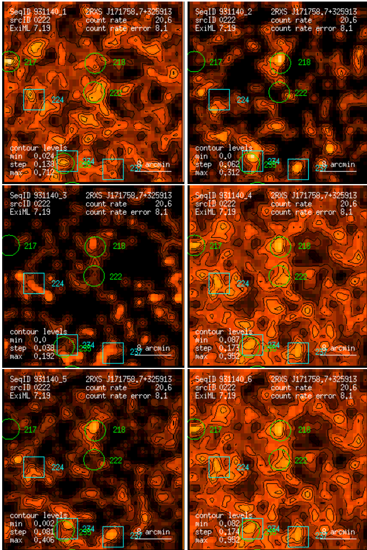
Figure 222: RASS 931140: detection 0222: band rate images, Gaussian filter: (1) PSPC channels 11 – 41, (2) 52 – 90, (3) 91 – 201, (4) 11 – 235, (5) 52 – 201, (6) 11 – 201. Broad band rates in counts/ks. Band rate contour levels in counts/ks/arcmin 2 .
