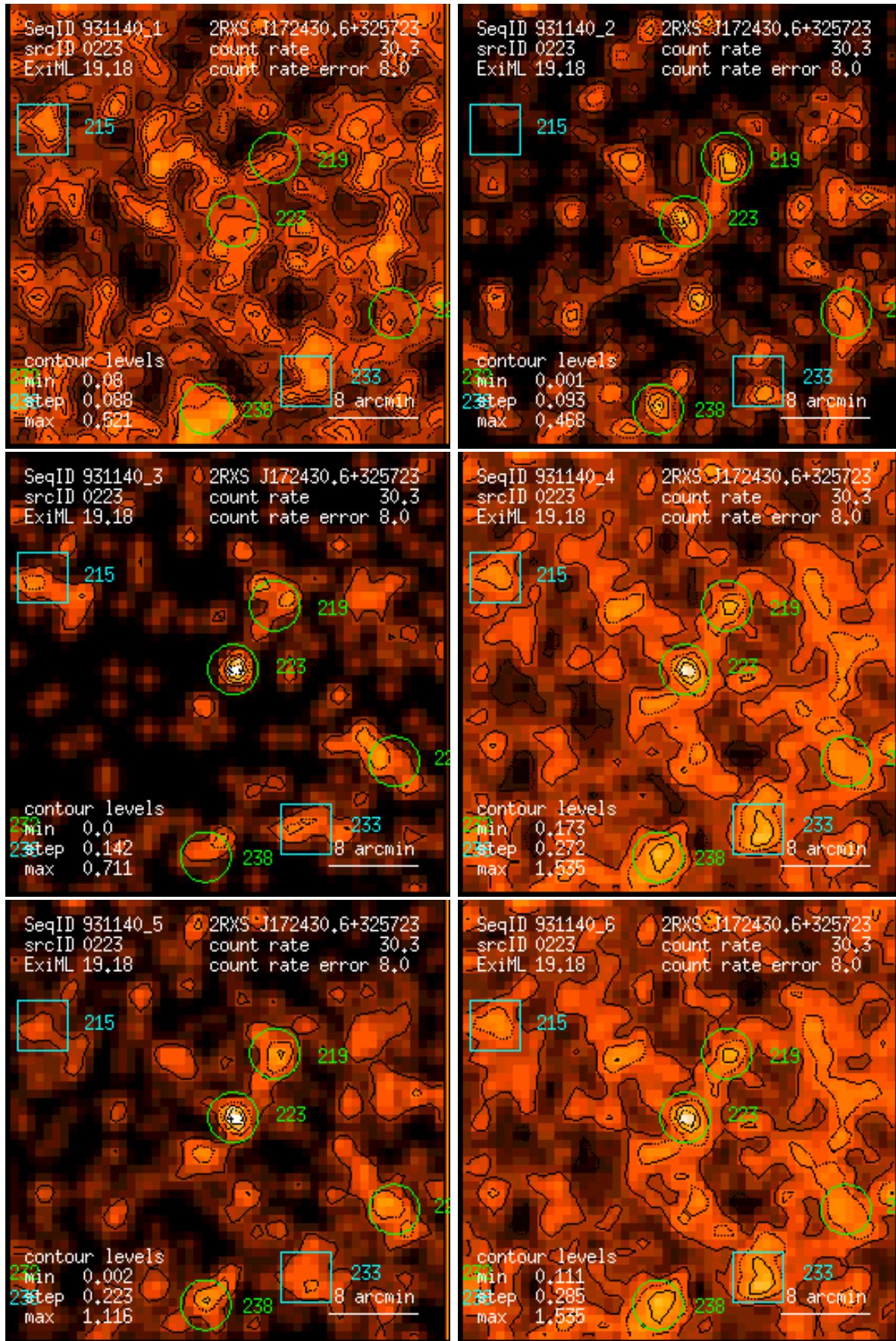
Figure 223: RASS 931140: detection 0223: band rate images, Gaussian filter: (1) PSPC channels 11 – 41, (2) 52 – 90, (3) 91 – 201, (4) 11 – 235, (5) 52 – 201, (6) 11 – 201. Broad band rates in counts/ks. Band rate contour levels in counts/ks/arcmin 2 .
