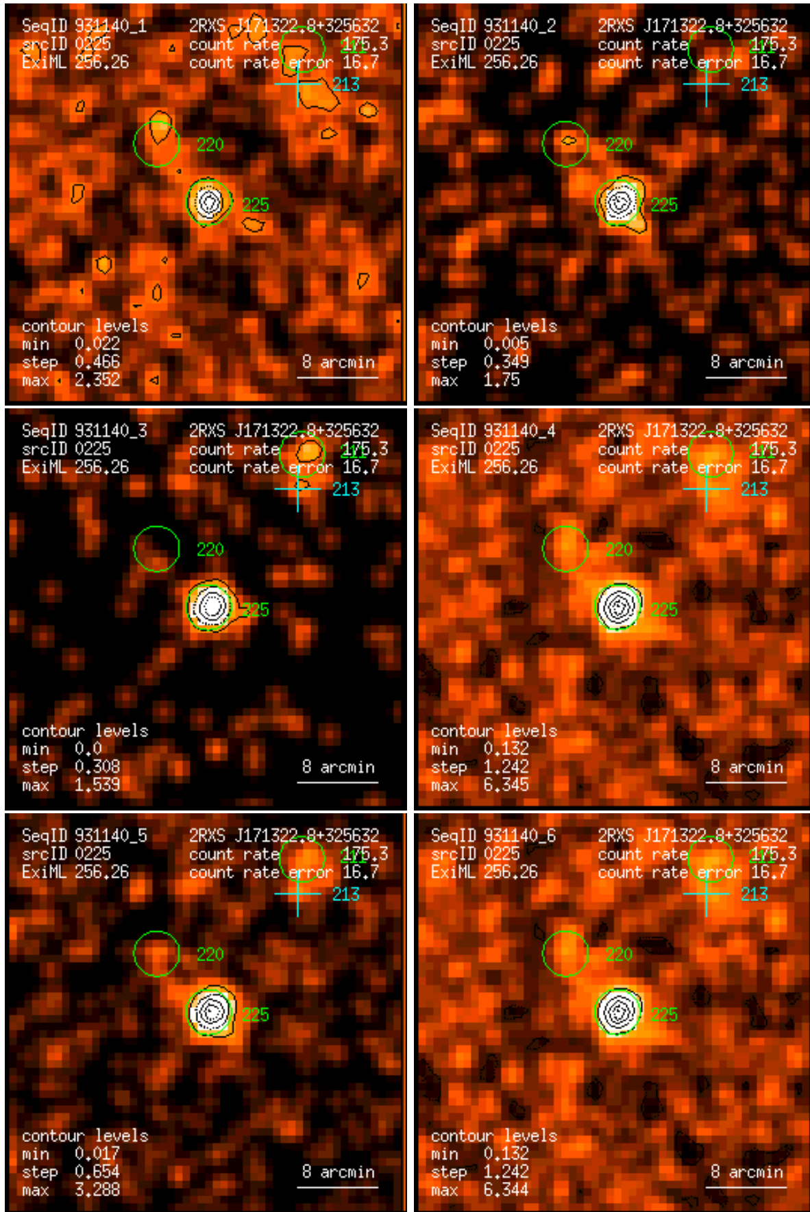
Figure 225: RASS 931140: detection 0225: band rate images, Gaussian filter: (1) PSPC channels 11 – 41, (2) 52 – 90, (3) 91 – 201, (4) 11 – 235, (5) 52 – 201, (6) 11 – 201. Broad band rates in counts/ks. Band rate contour levels in counts/ks/arcmin 2 .
