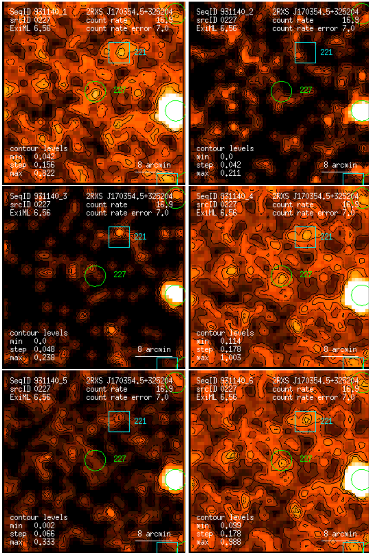
Figure 227: RASS 931140: detection 0227: band rate images, Gaussian filter: (1) PSPC channels 11 – 41, (2) 52 – 90, (3) 91 – 201, (4) 11 – 235, (5) 52 – 201, (6) 11 – 201. Broad band rates in counts/ks. Band rate contour levels in counts/ks/arcmin 2 .
