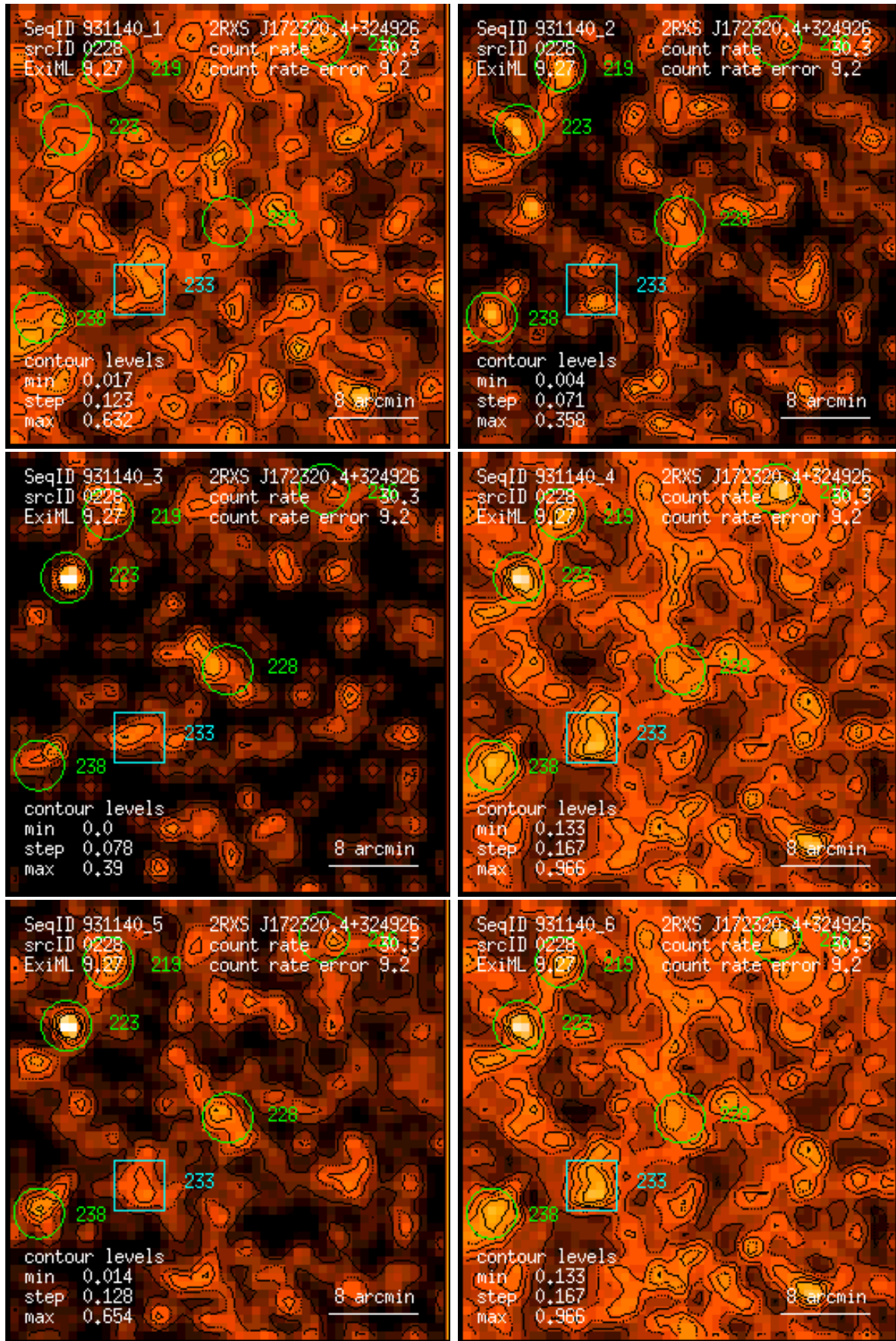
Figure 228: RASS 931140: detection 0228: band rate images, Gaussian filter: (1) PSPC channels 11 – 41, (2) 52 – 90, (3) 91 – 201, (4) 11 – 235, (5) 52 – 201, (6) 11 – 201. Broad band rates in counts/ks. Band rate contour levels in counts/ks/arcmin 2 .
