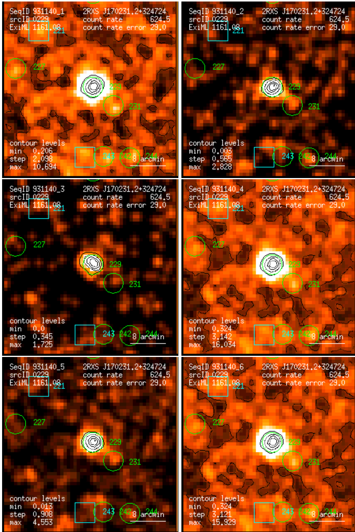
Figure 229: RASS 931140: detection 0229: band rate images, Gaussian filter: (1) PSPC channels 11 – 41, (2) 52 – 90, (3) 91 – 201, (4) 11 – 235, (5) 52 – 201, (6) 11 – 201. Broad band rates in counts/ks. Band rate contour levels in counts/ks/arcmin 2 .
