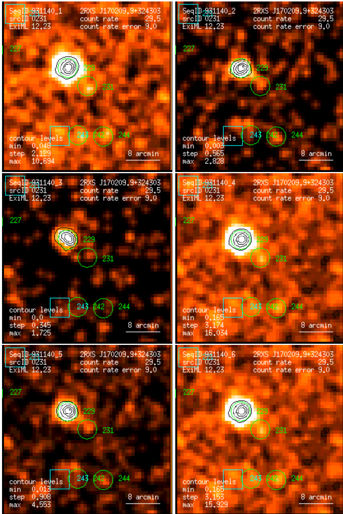
Figure 231: RASS 931140: detection 0231: band rate images, Gaussian filter: (1) PSPC channels 11 – 41, (2) 52 – 90, (3) 91 – 201, (4) 11 – 235, (5) 52 – 201, (6) 11 – 201. Broad band rates in counts/ks. Band rate contour levels in counts/ks/arcmin 2 .
