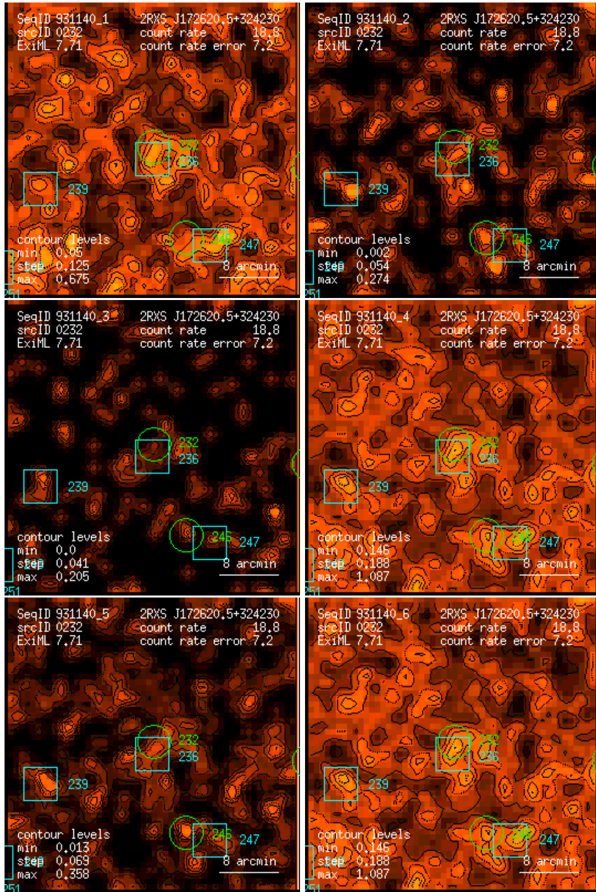
Figure 232: RASS 931140: detection 0232: band rate images, Gaussian filter: (1) PSPC channels 11 – 41, (2) 52 – 90, (3) 91 – 201, (4) 11 – 235, (5) 52 – 201, (6) 11 – 201. Broad band rates in counts/ks. Band rate contour levels in counts/ks/arcmin 2 .
