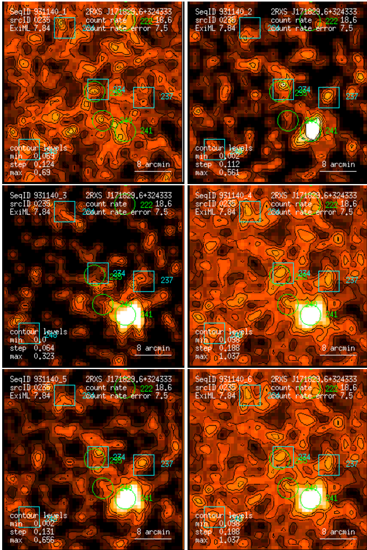
Figure 235: RASS 931140: detection 0235: band rate images, Gaussian filter: (1) PSPC channels 11 – 41, (2) 52 – 90, (3) 91 – 201, (4) 11 – 235, (5) 52 – 201, (6) 11 – 201. Broad band rates in counts/ks. Band rate contour levels in counts/ks/arcmin 2 .
