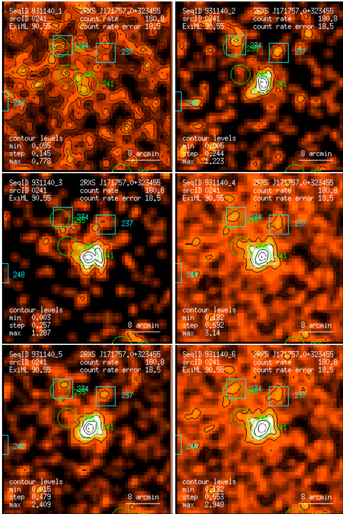
Figure 241: RASS 931140: detection 0241: band rate images, Gaussian filter: (1) PSPC channels 11 – 41, (2) 52 – 90, (3) 91 – 201, (4) 11 – 235, (5) 52 – 201, (6) 11 – 201. Broad band rates in counts/ks. Band rate contour levels in counts/ks/arcmin 2 .
