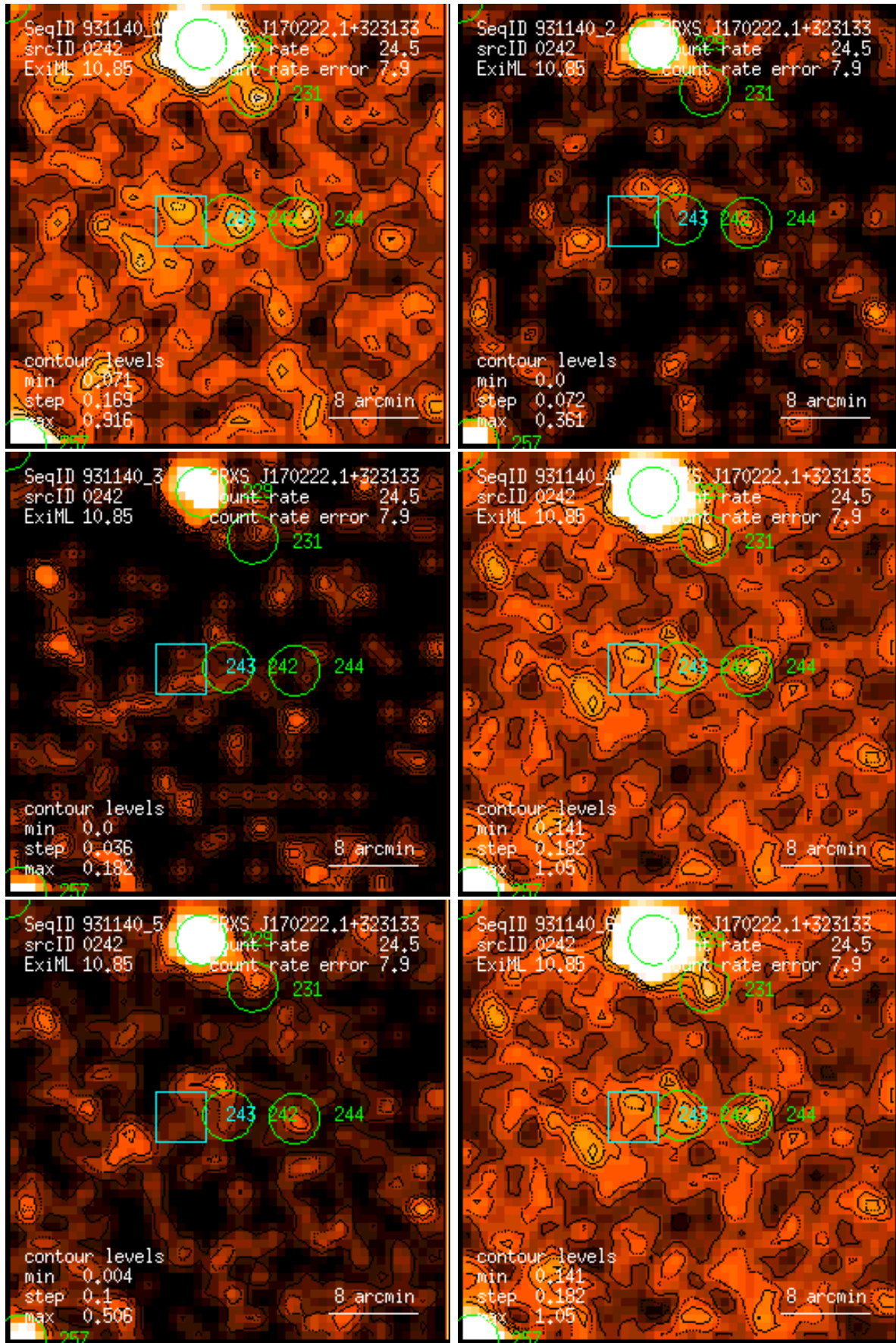
Figure 242: RASS 931140: detection 0242: band rate images, Gaussian filter: (1) PSPC channels 11 – 41, (2) 52 – 90, (3) 91 – 201, (4) 11 – 235, (5) 52 – 201, (6) 11 – 201. Broad band rates in counts/ks. Band rate contour levels in counts/ks/arcmin 2 .
