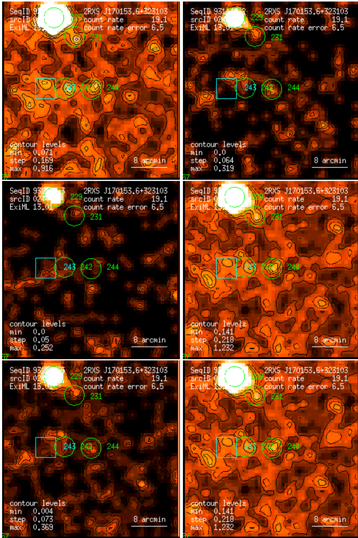
Figure 244: RASS 931140: detection 0244: band rate images, Gaussian filter: (1) PSPC channels 11 – 41, (2) 52 – 90, (3) 91 – 201, (4) 11 – 235, (5) 52 – 201, (6) 11 – 201. Broad band rates in counts/ks. Band rate contour levels in counts/ks/arcmin 2 .
