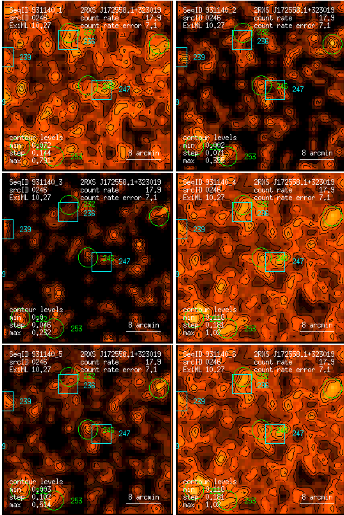
Figure 246: RASS 931140: detection 0246: band rate images, Gaussian filter: (1) PSPC channels 11 – 41, (2) 52 – 90, (3) 91 – 201, (4) 11 – 235, (5) 52 – 201, (6) 11 – 201. Broad band rates in counts/ks. Band rate contour levels in counts/ks/arcmin 2 .
