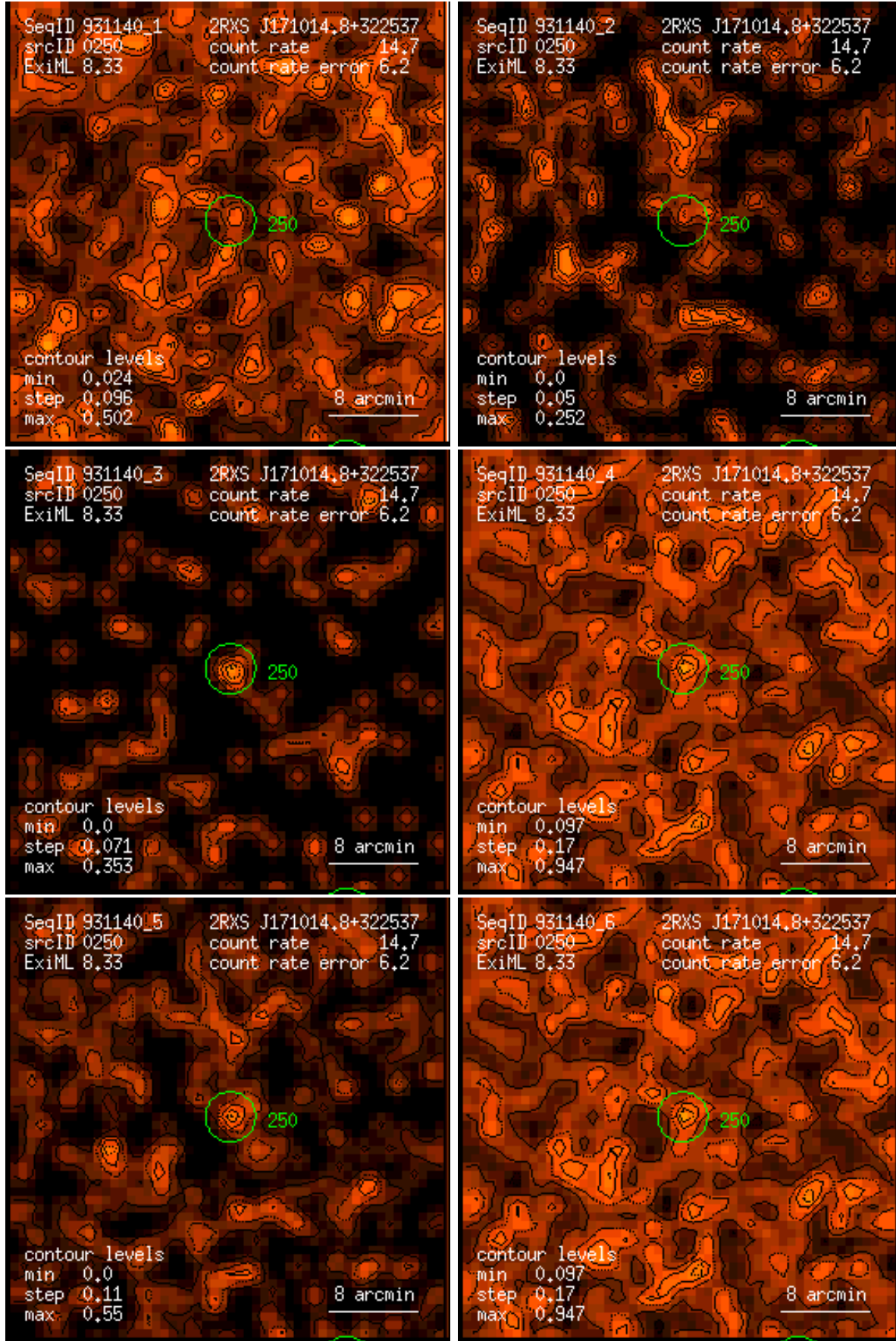
Figure 250: RASS 931140: detection 0250: band rate images, Gaussian filter: (1) PSPC channels 11 – 41, (2) 52 – 90, (3) 91 – 201, (4) 11 – 235, (5) 52 – 201, (6) 11 – 201. Broad band rates in counts/ks. Band rate contour levels in counts/ks/arcmin 2 .
