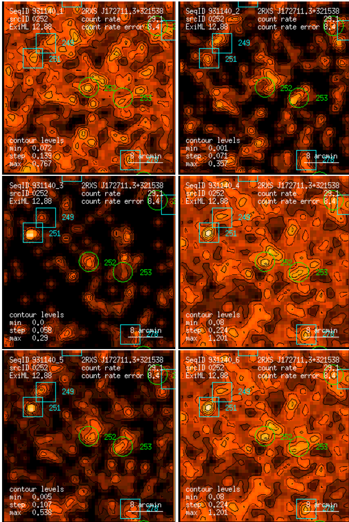
Figure 252: RASS 931140: detection 0252: band rate images, Gaussian filter: (1) PSPC channels 11 – 41, (2) 52 – 90, (3) 91 – 201, (4) 11 – 235, (5) 52 – 201, (6) 11 – 201. Broad band rates in counts/ks. Band rate contour levels in counts/ks/arcmin 2 .
