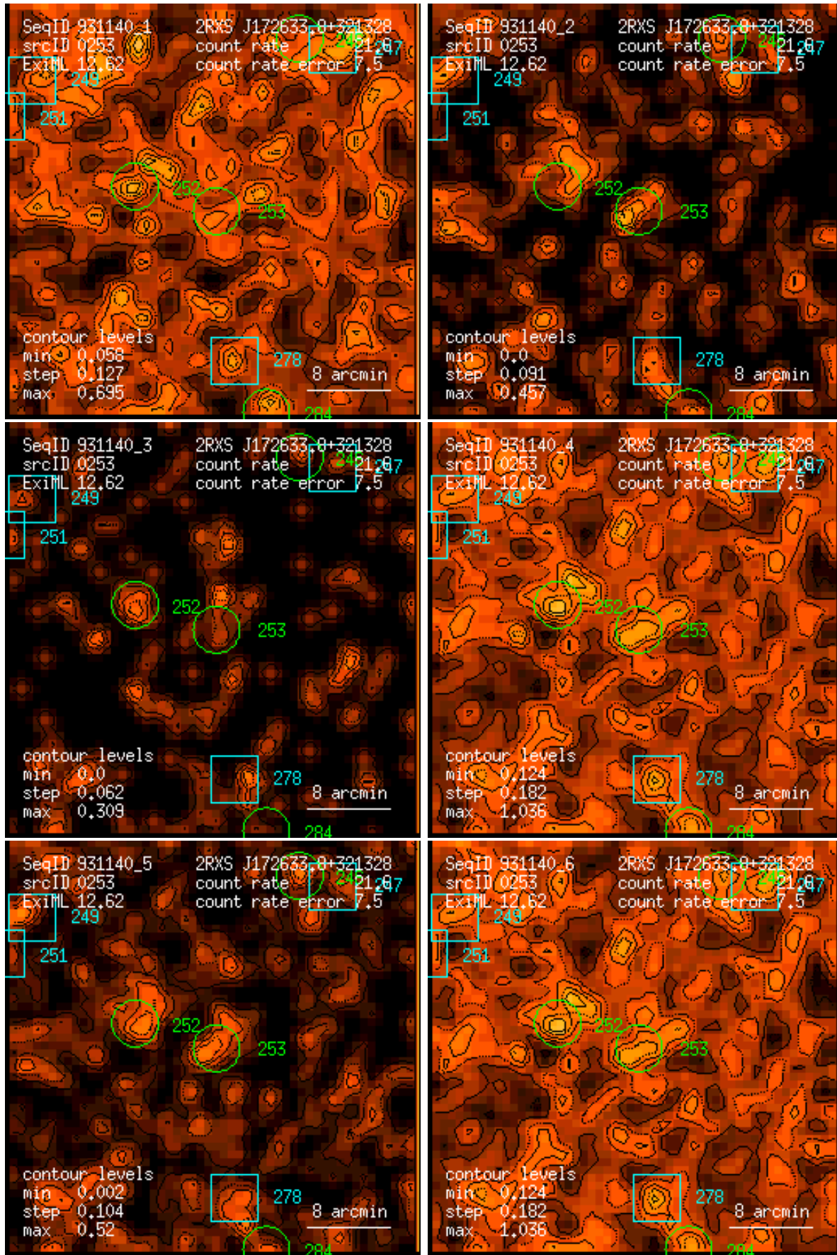
Figure 253: RASS 931140: detection 0253: band rate images, Gaussian filter: (1) PSPC channels 11 – 41, (2) 52 – 90, (3) 91 – 201, (4) 11 – 235, (5) 52 – 201, (6) 11 – 201. Broad band rates in counts/ks. Band rate contour levels in counts/ks/arcmin 2 .
