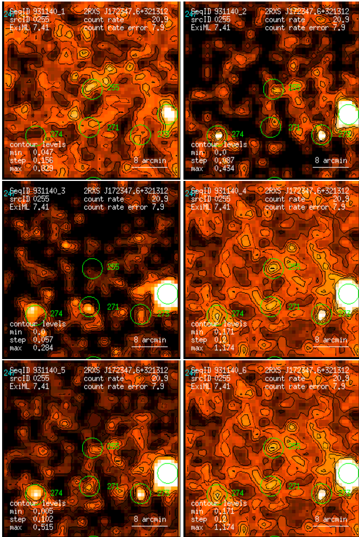
Figure 255: RASS 931140: detection 0255: band rate images, Gaussian filter: (1) PSPC channels 11 – 41, (2) 52 – 90, (3) 91 – 201, (4) 11 – 235, (5) 52 – 201, (6) 11 – 201. Broad band rates in counts/ks. Band rate contour levels in counts/ks/arcmin 2 .
