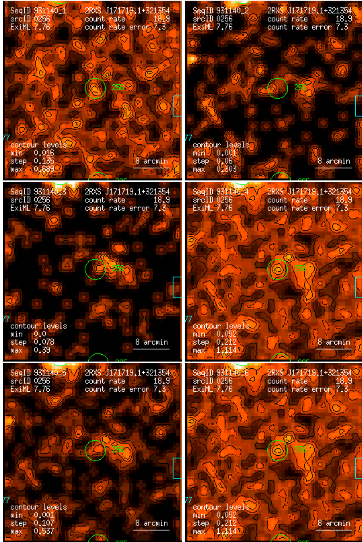
Figure 256: RASS 931140: detection 0256: band rate images, Gaussian filter: (1) PSPC channels 11 – 41, (2) 52 – 90, (3) 91 – 201, (4) 11 – 235, (5) 52 – 201, (6) 11 – 201. Broad band rates in counts/ks. Band rate contour levels in counts/ks/arcmin 2 .
