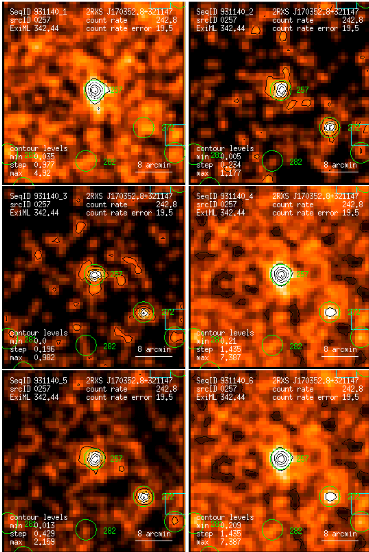
Figure 257: RASS 931140: detection 0257: band rate images, Gaussian filter: (1) PSPC channels 11 – 41, (2) 52 – 90, (3) 91 – 201, (4) 11 – 235, (5) 52 – 201, (6) 11 – 201. Broad band rates in counts/ks. Band rate contour levels in counts/ks/arcmin 2 .
