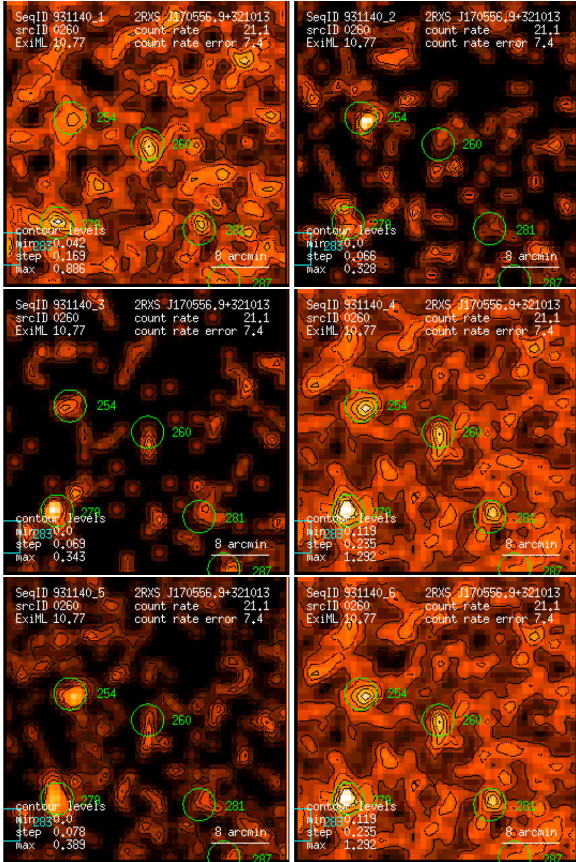
Figure 260: RASS 931140: detection 0260: band rate images, Gaussian filter: (1) PSPC channels 11 – 41, (2) 52 – 90, (3) 91 – 201, (4) 11 – 235, (5) 52 – 201, (6) 11 – 201. Broad band rates in counts/ks. Band rate contour levels in counts/ks/arcmin 2 .
