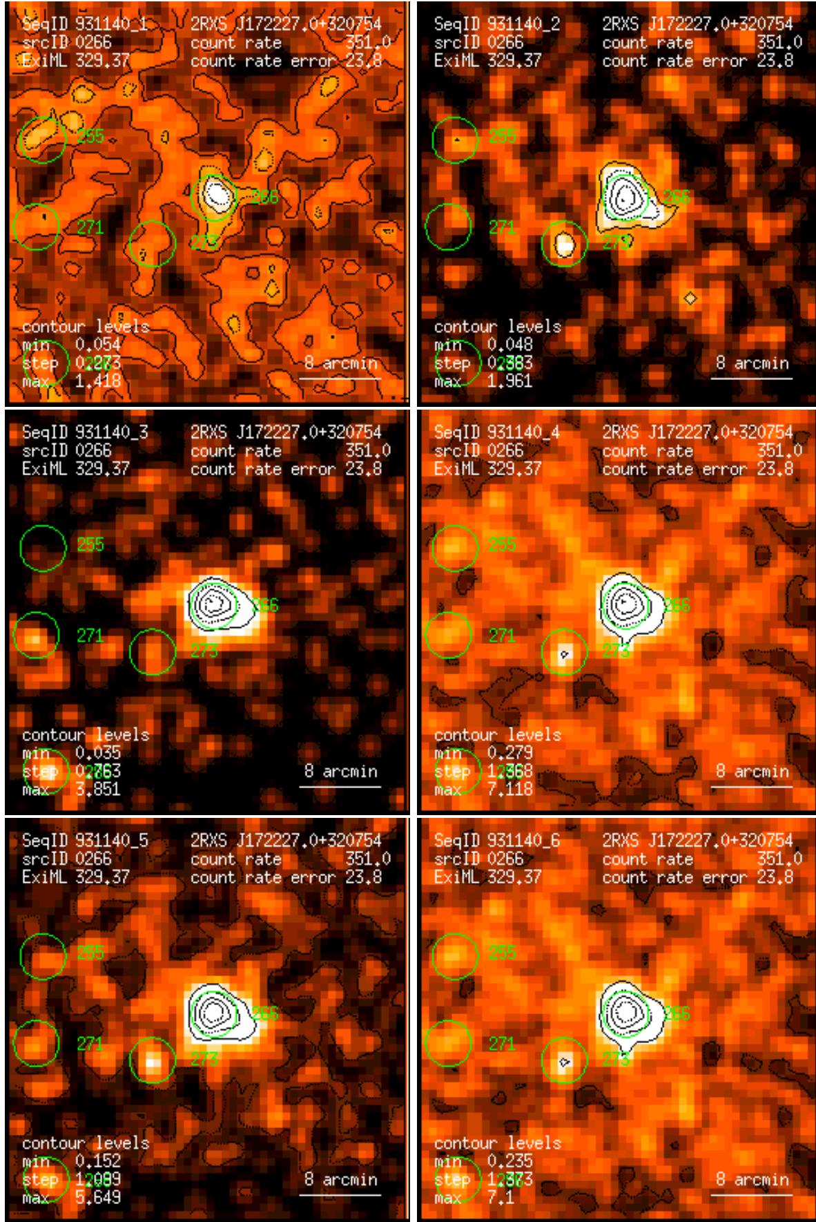
Figure 266: RASS 931140: detection 0266: band rate images, Gaussian filter: (1) PSPC channels 11 – 41, (2) 52 – 90, (3) 91 – 201, (4) 11 – 235, (5) 52 – 201, (6) 11 – 201. Broad band rates in counts/ks. Band rate contour levels in counts/ks/arcmin 2 .
