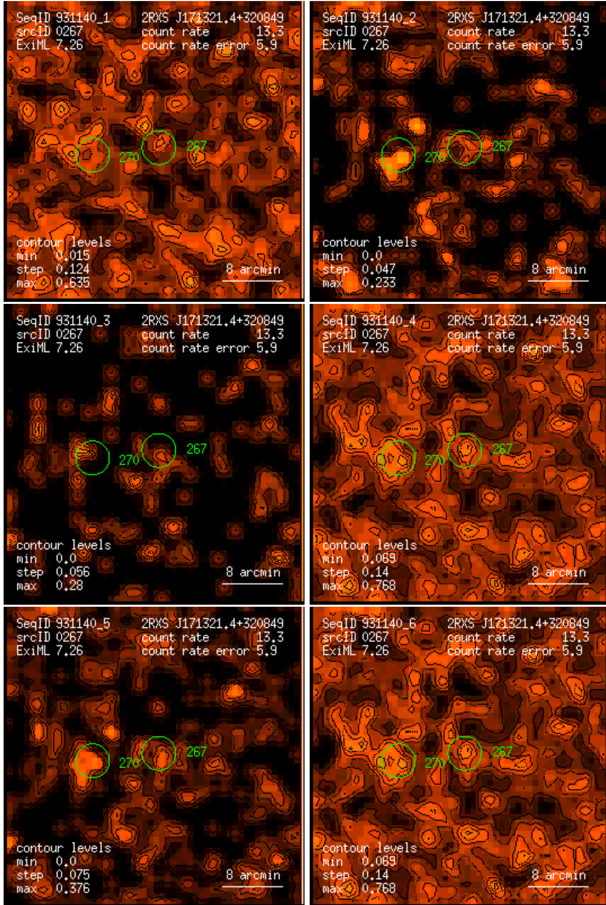
Figure 267: RASS 931140: detection 0267: band rate images, Gaussian filter: (1) PSPC channels 11 – 41, (2) 52 – 90, (3) 91 – 201, (4) 11 – 235, (5) 52 – 201, (6) 11 – 201. Broad band rates in counts/ks. Band rate contour levels in counts/ks/arcmin 2 .
