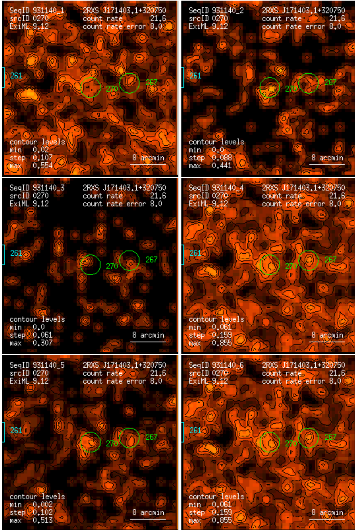
Figure 270: RASS 931140: detection 0270: band rate images, Gaussian filter: (1) PSPC channels 11 – 41, (2) 52 – 90, (3) 91 – 201, (4) 11 – 235, (5) 52 – 201, (6) 11 – 201. Broad band rates in counts/ks. Band rate contour levels in counts/ks/arcmin 2 .
